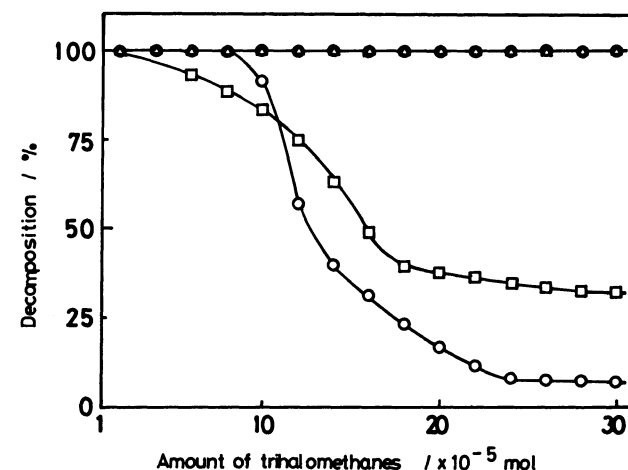
□: \text{CH}_2\text{Cl}_2 , ○: \text{CHCl}_3 , ●: \text{CHClBr}_2 , △: \text{CHBr}_3
